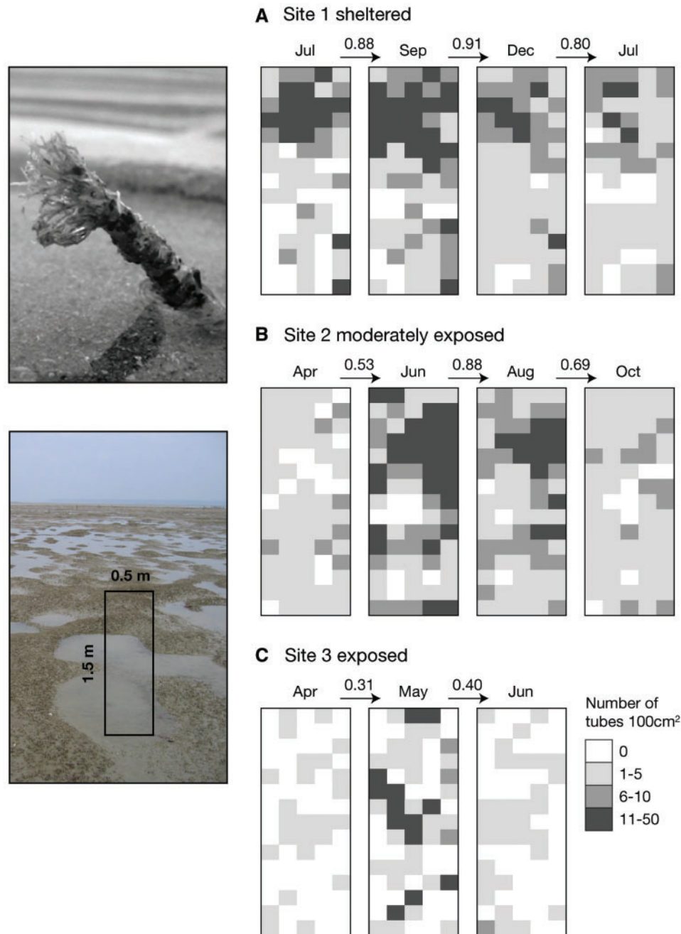
Fig. 2 Small-scale distribution of L. conchilega within fixed 0.5 \times 1.5 m plots at three differently exposed sites. Densities of L. conchilega tubes in 100\text{-cm}^2 grid cells are shown. (A) Site 1 was in the Wadden Sea (Germany) and monitored four times over 1 year; (B) Site 2 was in Swansea Bay (Wales, UK) and monitored over 7 months. (C) Site 3 was in Rhossili Bay (Wales, UK) monitored over 3 months. The cosine similarity index between consecutive monitoring dates is given. One plot per site is shown. Images on the left show a single L. conchilega tube (top) and L. conchilega aggregations with a schematic monitoring plot (bottom).
